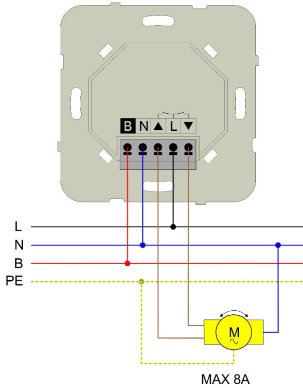
Connection Diagram:
