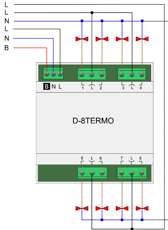
Connection Diagram:
