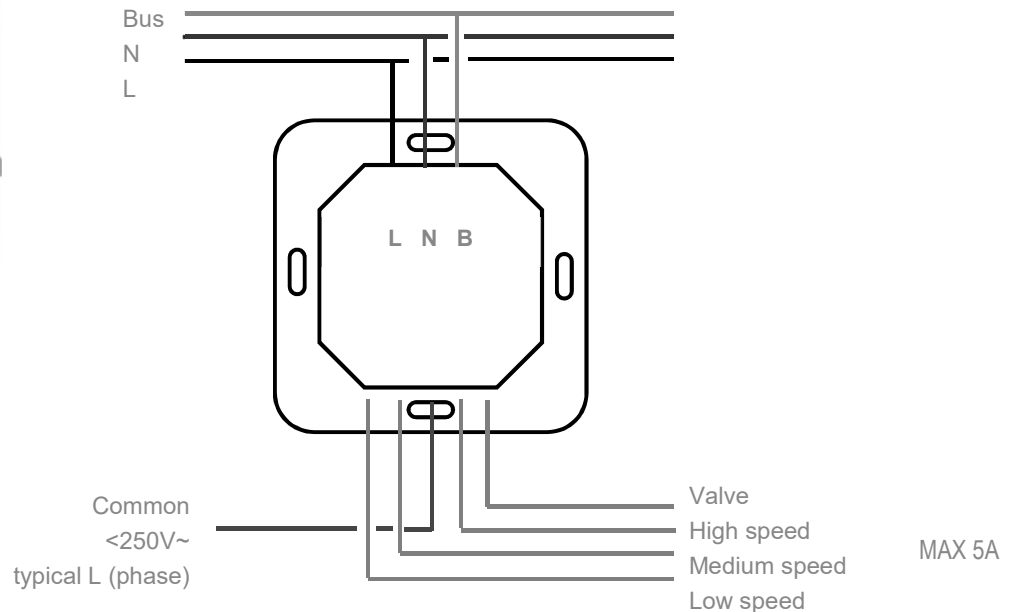
Connection Diagram:
