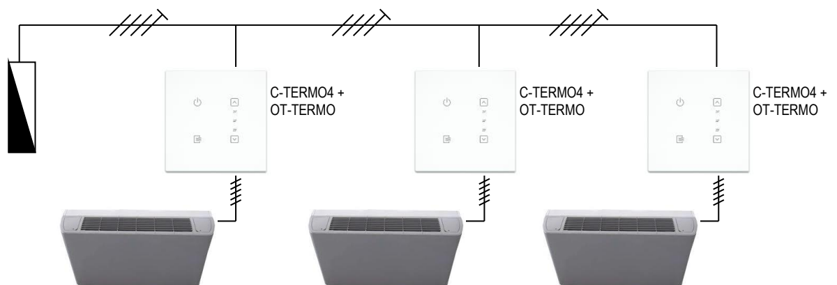
Fig: climatization by fan coil units
